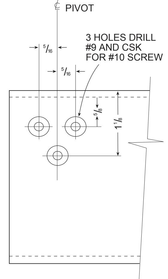
1422 ROUTER DRILL JIG TEMPLATE CUT OUT & HOLE PATTERN AMARLITE
