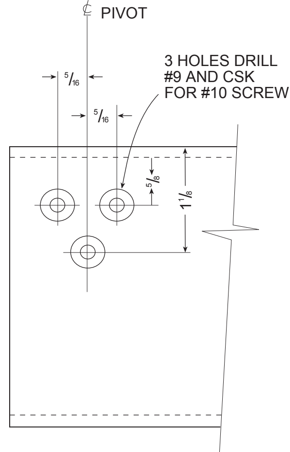
1412 ROUTER DRILL JIG TEMPLATE CUT OUT & HOLE PATTERN ALDORA
