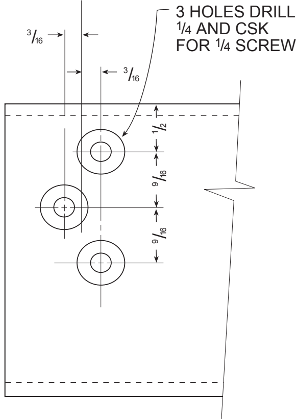
1442 ROUTER DRILL JIG TEMPLATE CUT OUT & HOLE PATTERN EXTRUDART
