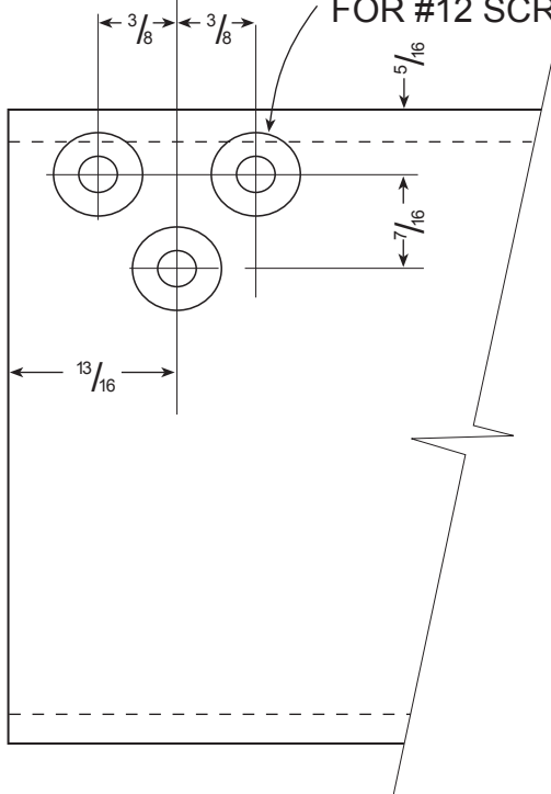
1417 ROUTER DRILL JIG TEMPLATE CUT OUT & HOLE PATTERN JACKSON SEE NOTE PAGE E-1
