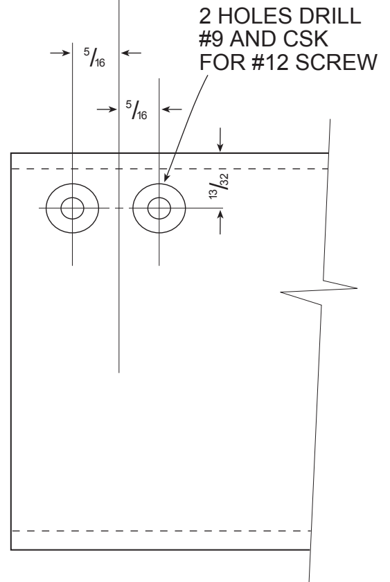
1447 ROUTER DRILL JIG TEMPLATE CUT OUT & HOLE PATTERN U. S. ALUMINUM
