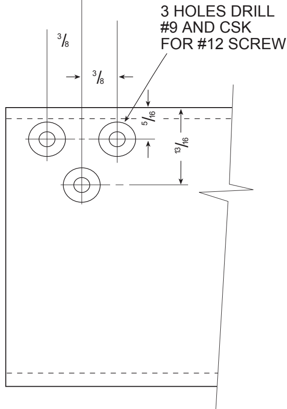
1432 ROUTER DRILL JIG TEMPLATE CUT OUT & HOLE PATTERN HOWMET VISTAWALL
