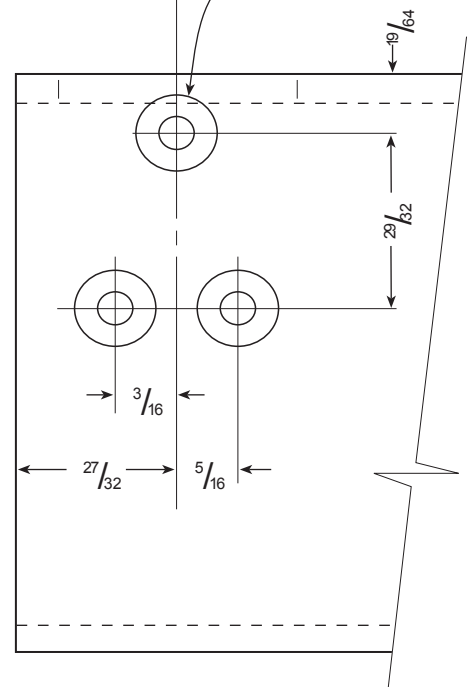
1437 ROUTER DRILL JIG TEMPLATE CUT OUT & HOLE PATTERN KAWNEER
